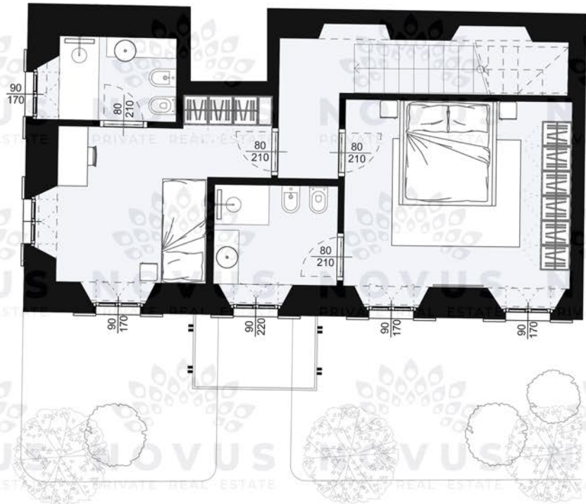
PIANO TERRA
